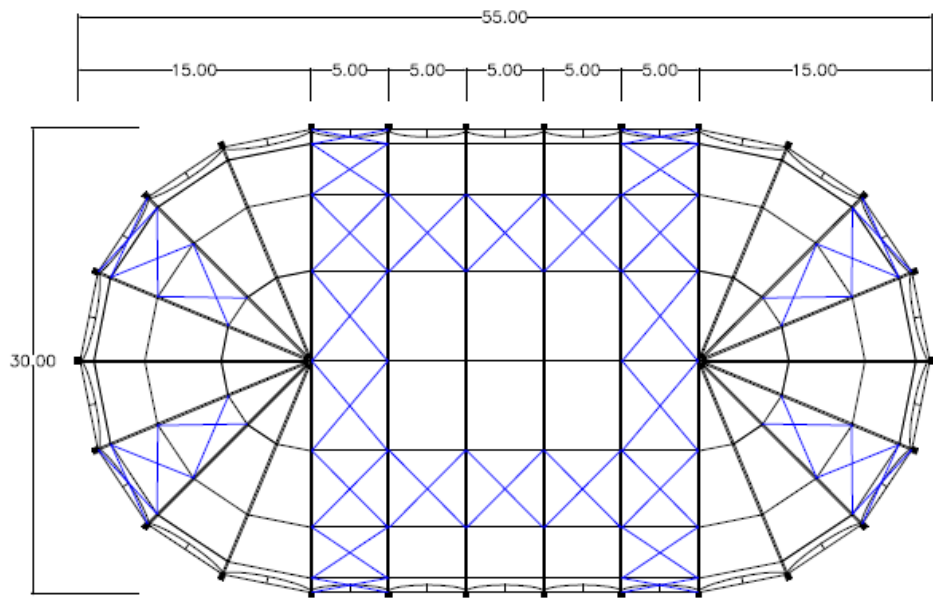
TOP VIEW
